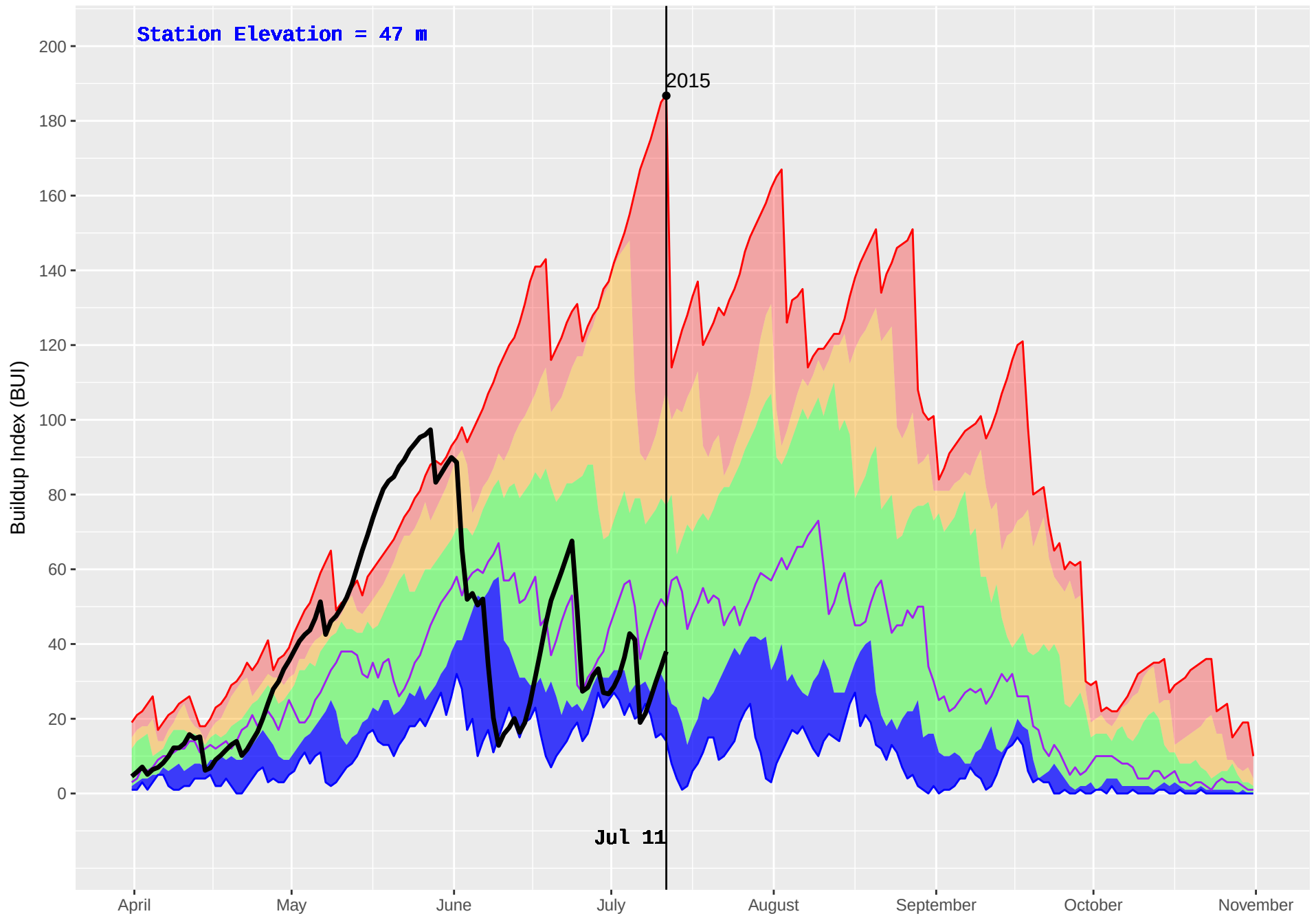
HAGENSBORG 2 (904) : Historical (2005–2016) and Current (2018) Noon Buildup Index (BUI)
