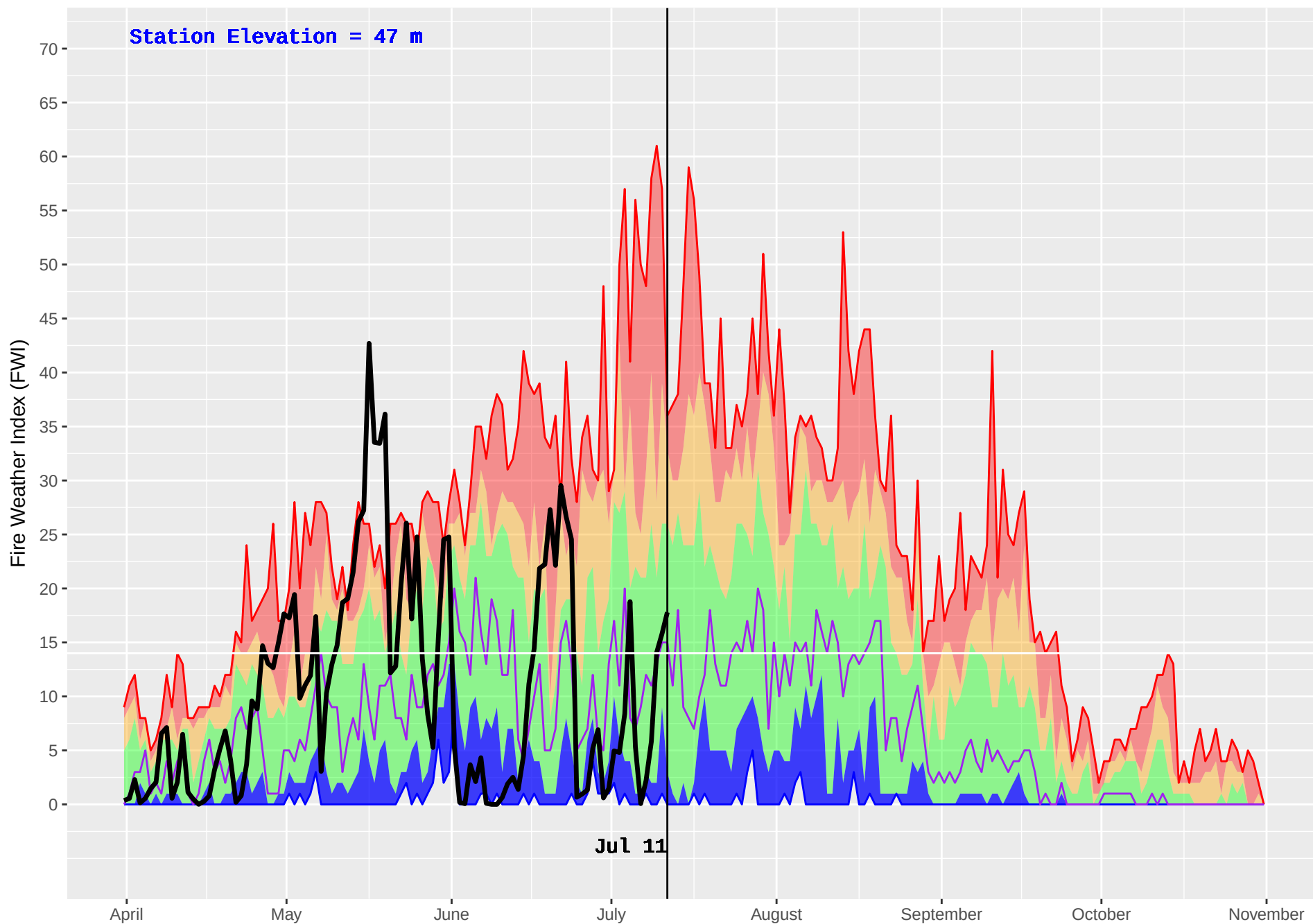
HAGENSBORG 2 (904) : Historical (2005–2016) and Current (2018) Noon Fire Weather Index (FWI)
