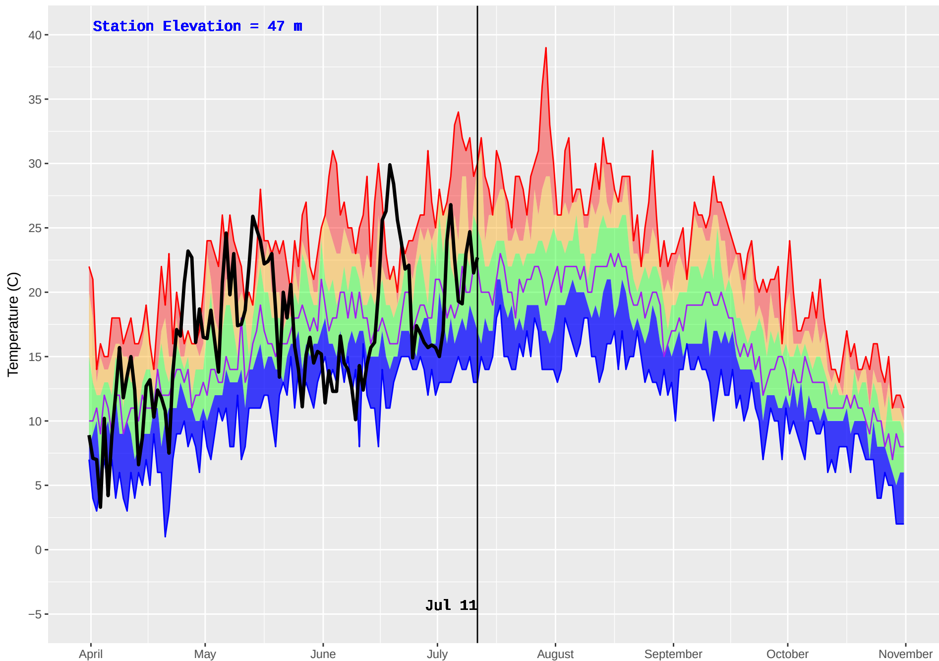
HAGENSBORG 2 (904) : Historical (2005–2016) and Current (2018) Noon Temperature
