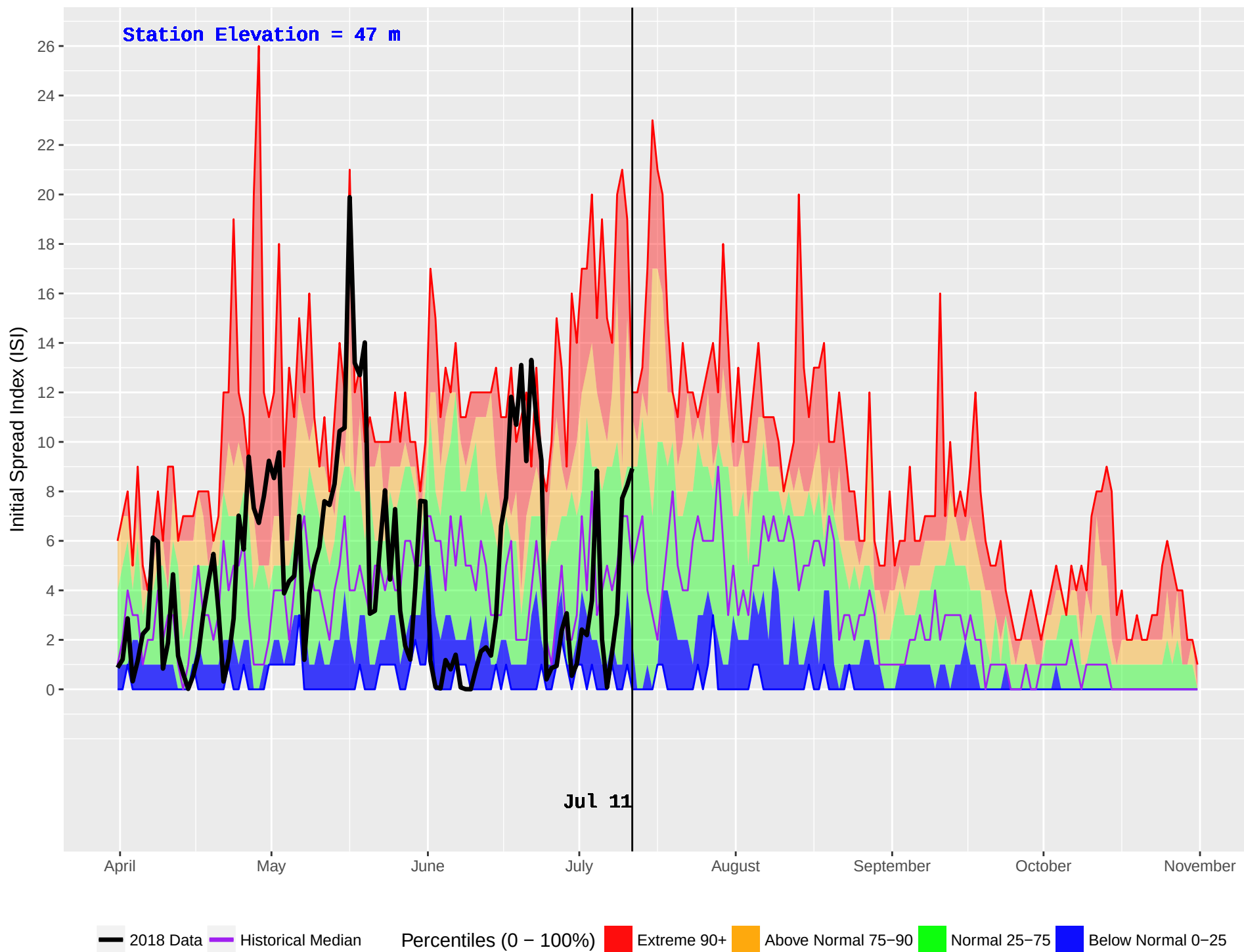
HAGENSBORG 2 (904) : Historical (2005–2016) and Current (2018) Noon Initial Spread Index (ISI)
