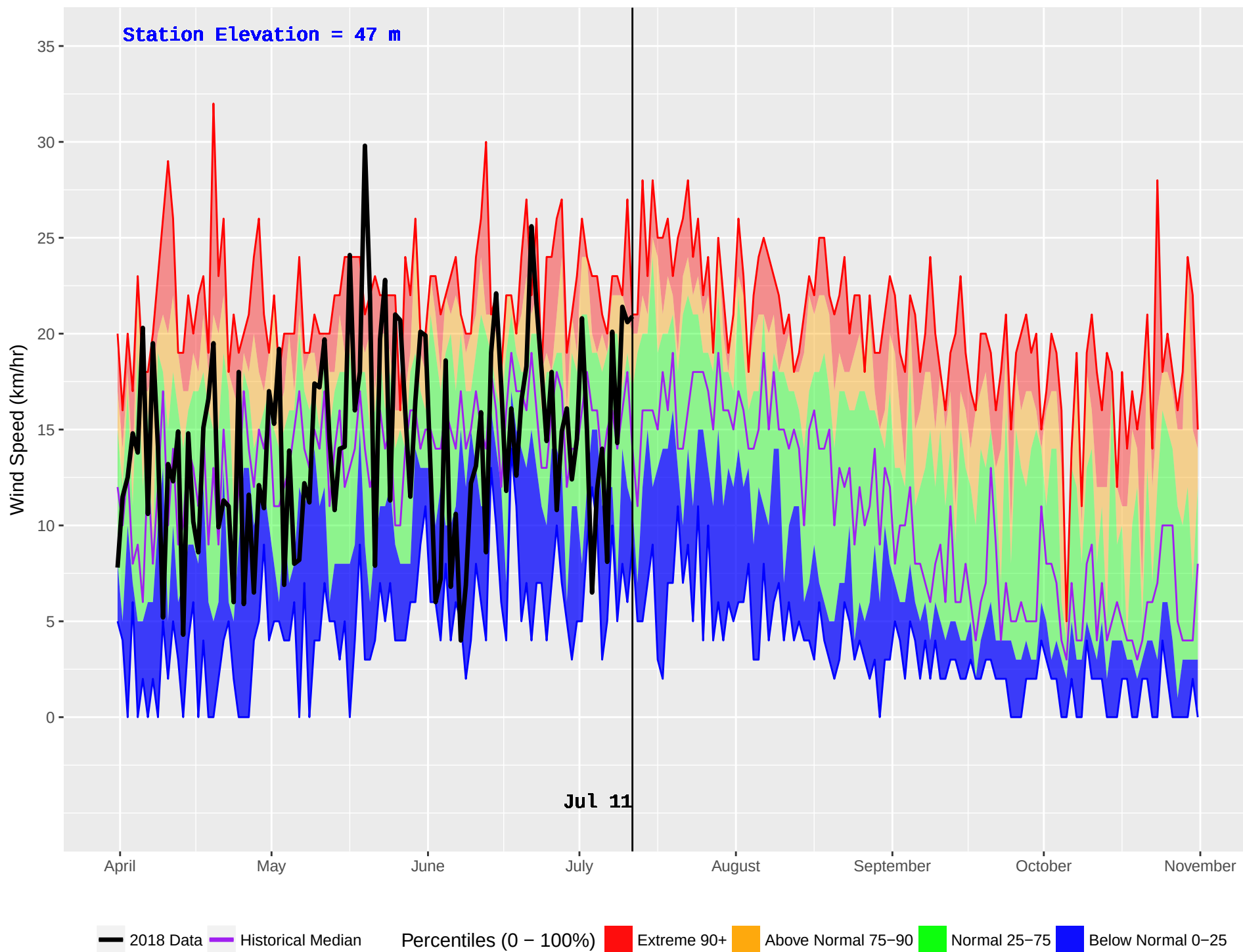
HAGENSBORG 2 (904) : Historical (2005–2016) and Current (2018) Noon Wind Speed
